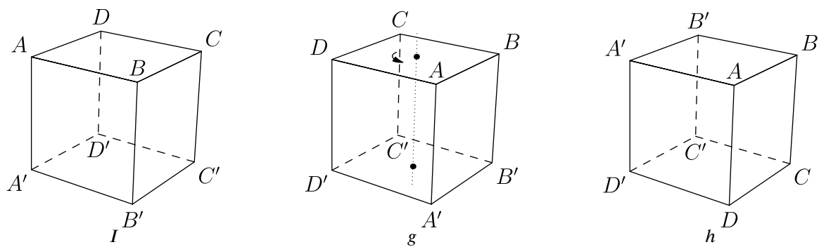
Figure 15: Elements g and h . Note that h is not solely a reflection about a mirror plane, but actually a combination of a rotation and reflection: a so-called rotoinversion!
